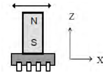
Figure 27: Orientation of the magnet for back-biasing the GMR sensor, (Source: NVE Corporation)
