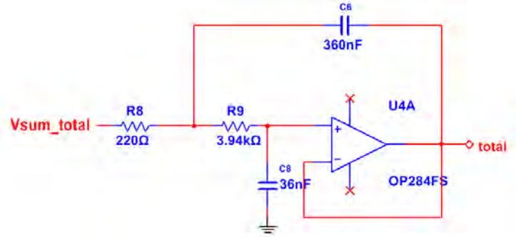
Figure 54: 2th Order Sallen-key LPF of the final GMR pickup circuit design
