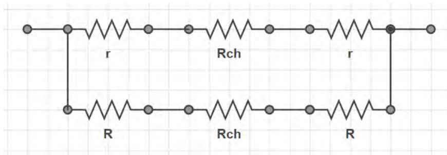
Figure 10: Schematic for Parallel Inter-layer Resistances
