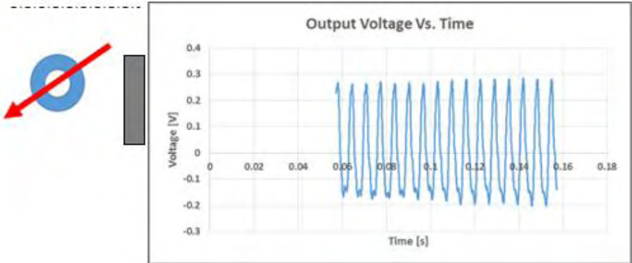
Figure 35: Graph for Output Voltage when the angle between the positive x-axis and the magnet's North Pole is 225 degrees
