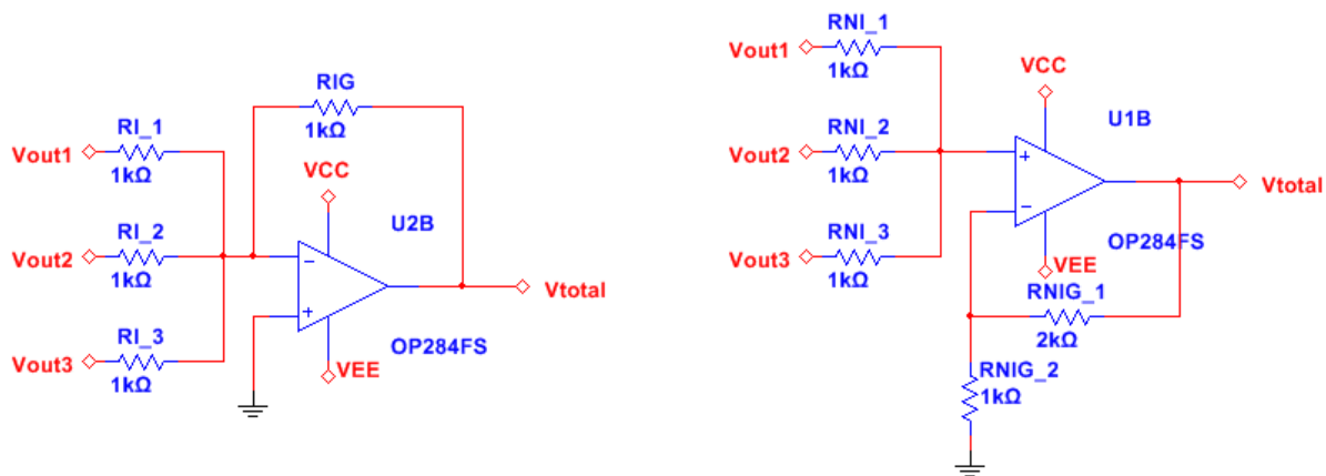
Figure 53: Inverting Vs non-inverting op-amp summing amplifiers
